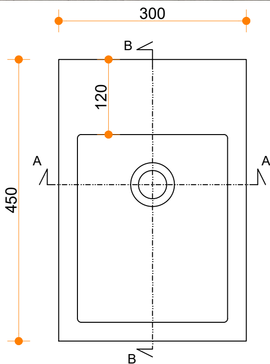
PLAN VIEW
