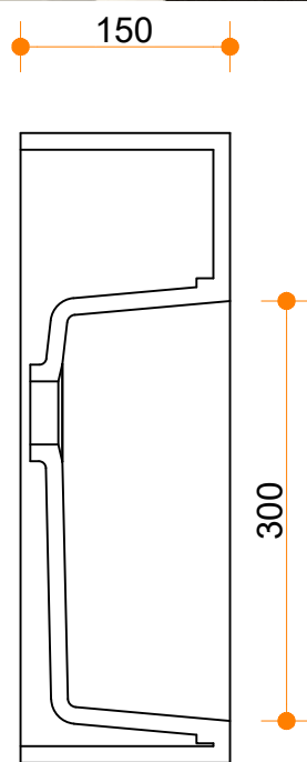
SECTION B:B
