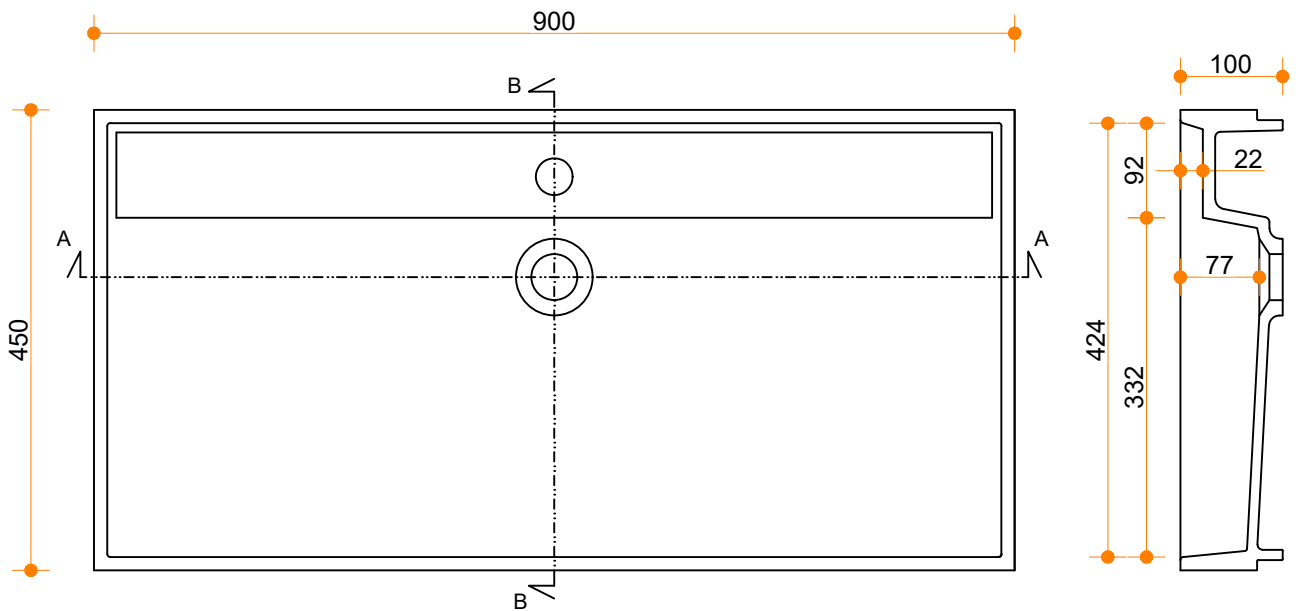
PLAN VIEW
